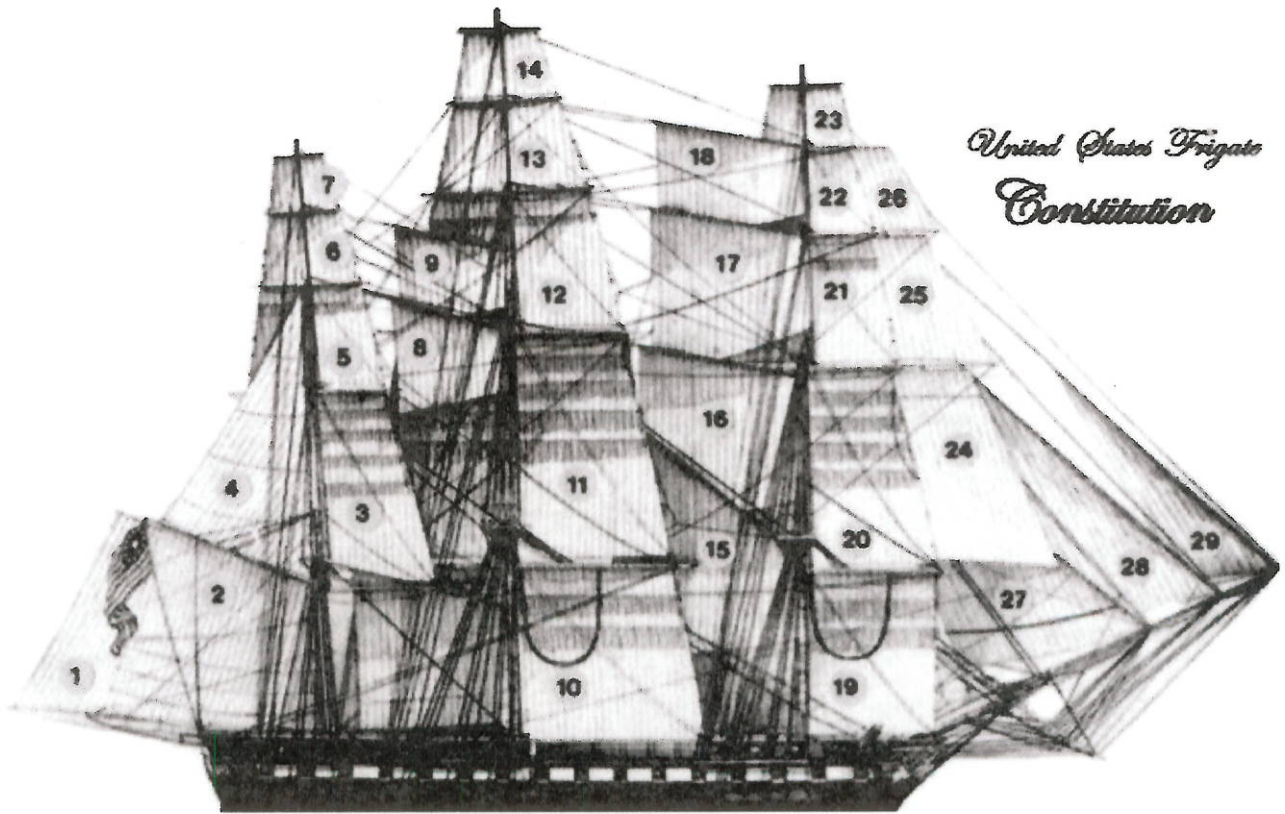
Sail Plan United States Frigate Constitution
